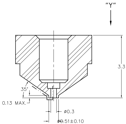
SECTION X-X
